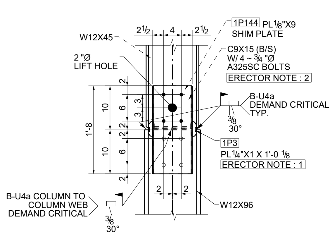
TYPICAL W12X96 COLUMN TO W12X45 COLUMN SPLICE CONNECTION DETAILS @ BRACE LOCATION
