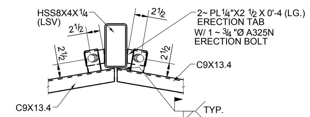
SECTION H - H
