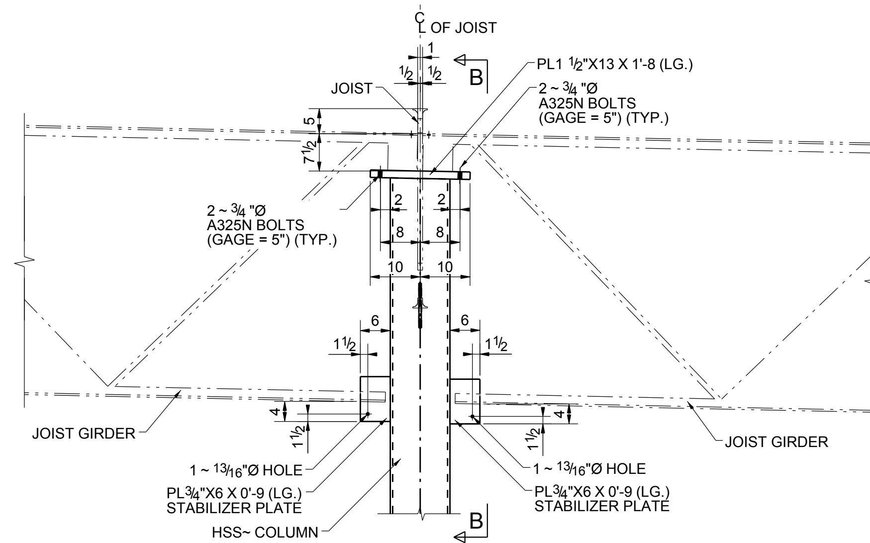
TYPICAL JOIST GIRDER RESTING ABOVE HSS ~ COLUMN TIE JOIST CONNECTION DETAIL
