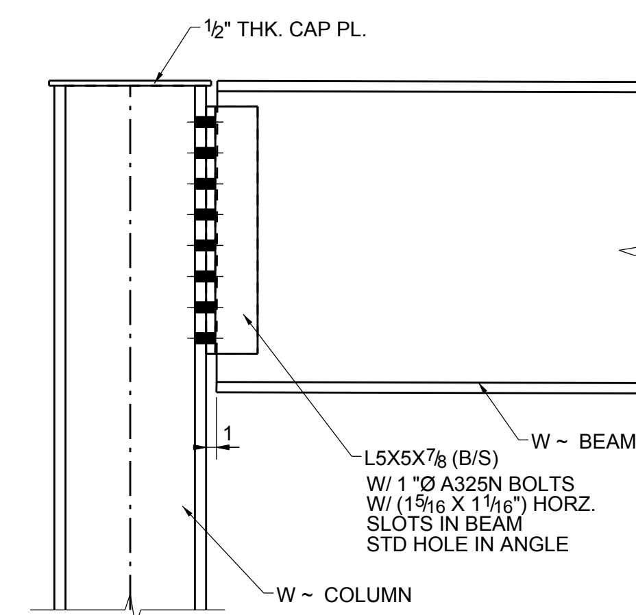
TYPICAL W ~ BEAM TO W ~ COLUMN KNIFE ANGLE CONNECTION DETAIL ALONG GRID LINE "16"
