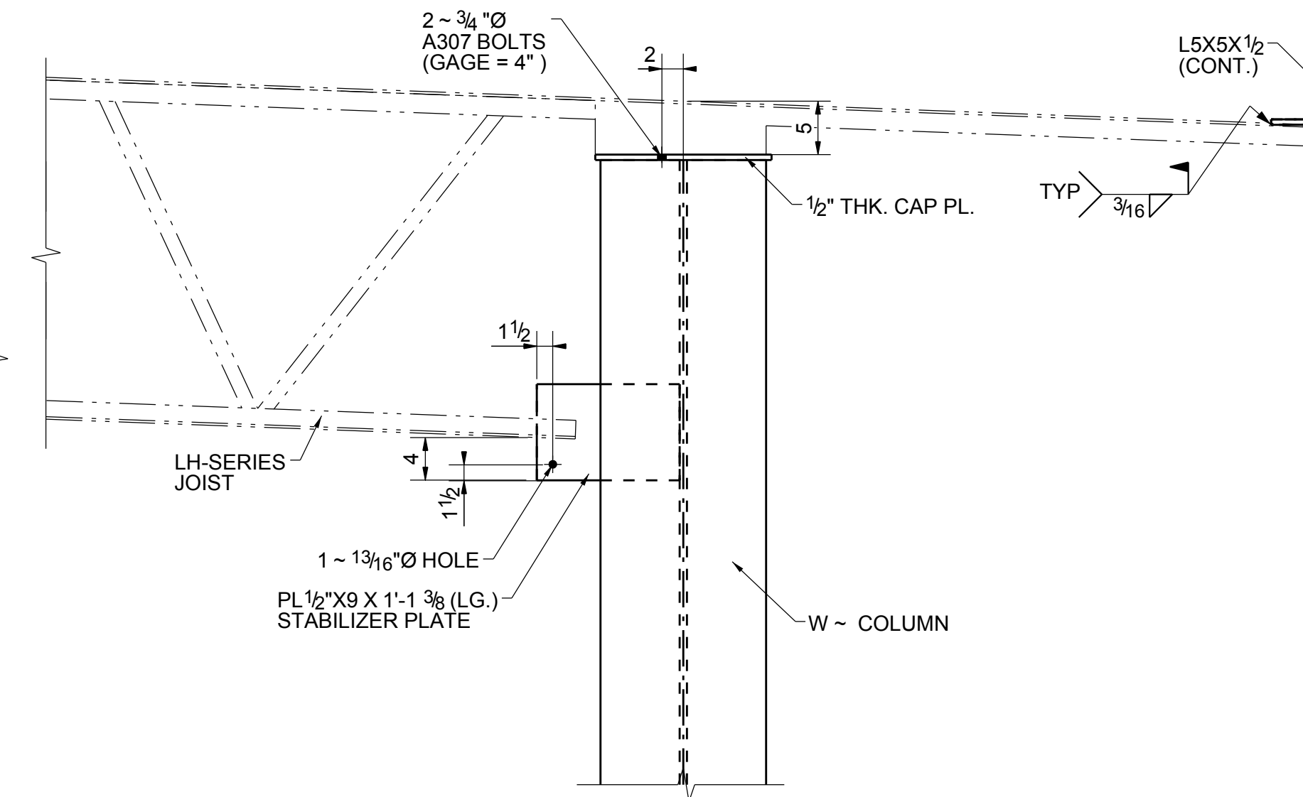
TYPICAL JOIST TO W ~ COLUMN WEB TIE JOIST CONNECTION DETAIL
