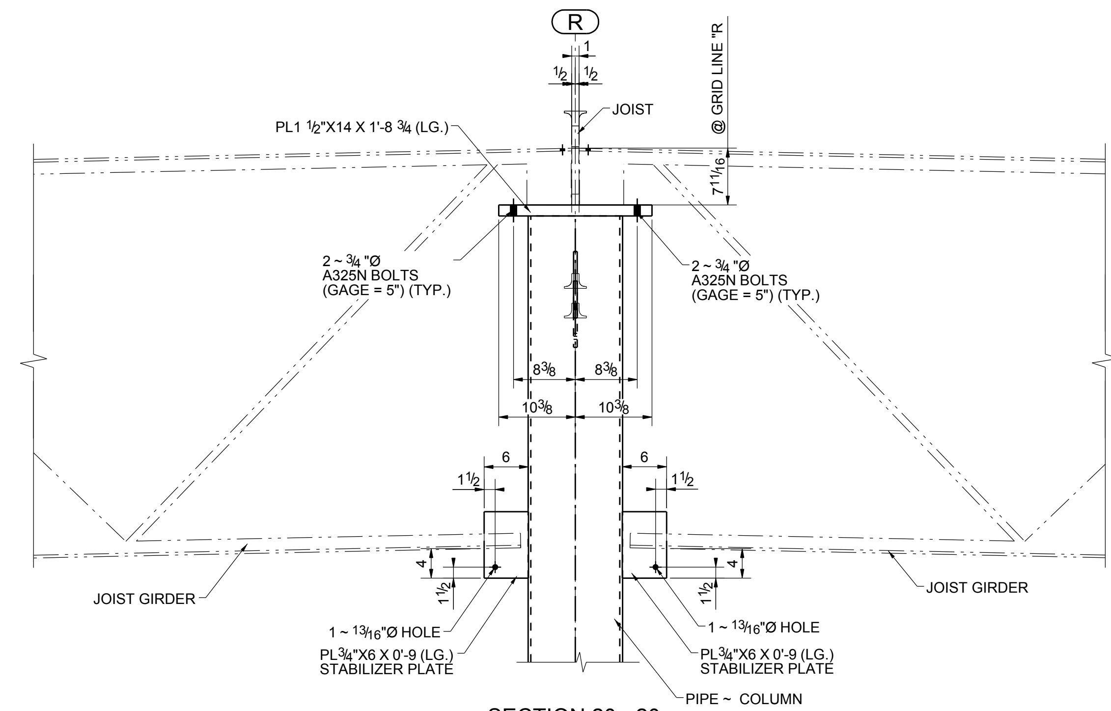
SECTION 20 - 20 E102 TYPICAL JOIST GIRDER RESTING ABOVE PIPE ~ COLUMN TIE JOIST CONNECTION DETAIL ALONG GRID LINE "R"
