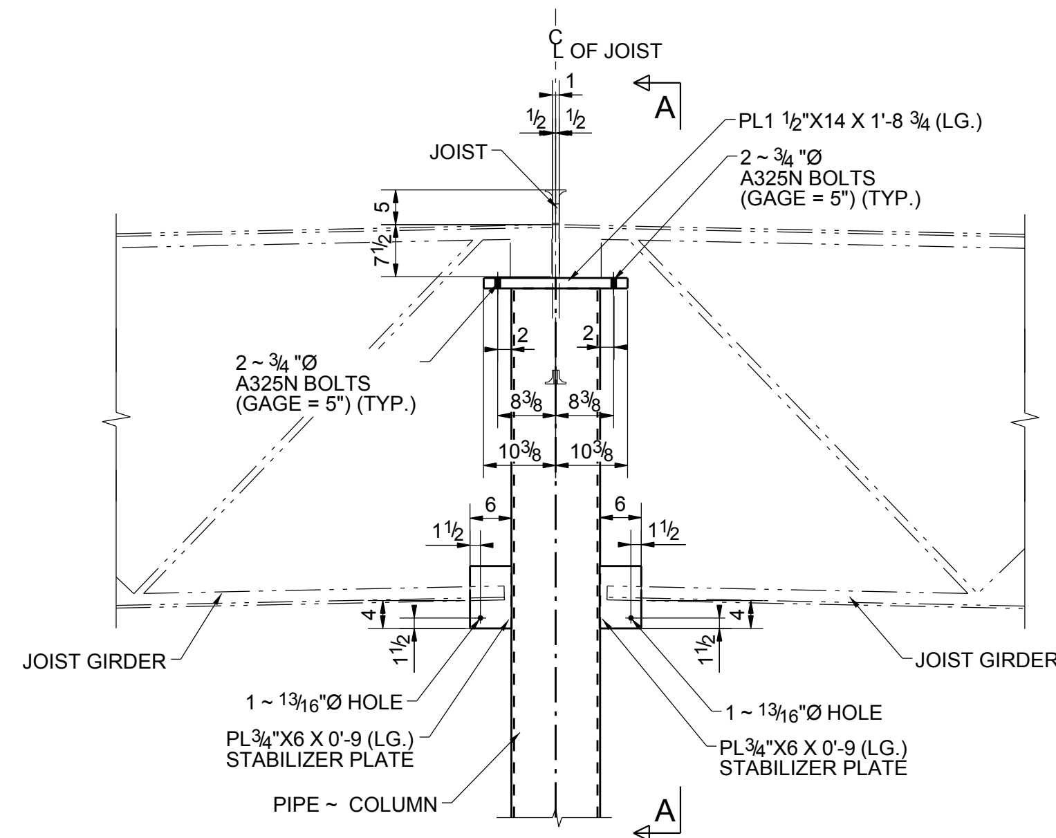
TYPICAL JOIST GIRDER RESTING ABOVE PIPE ~ COLUMN TIE JOIST CONNECTION DETAIL
