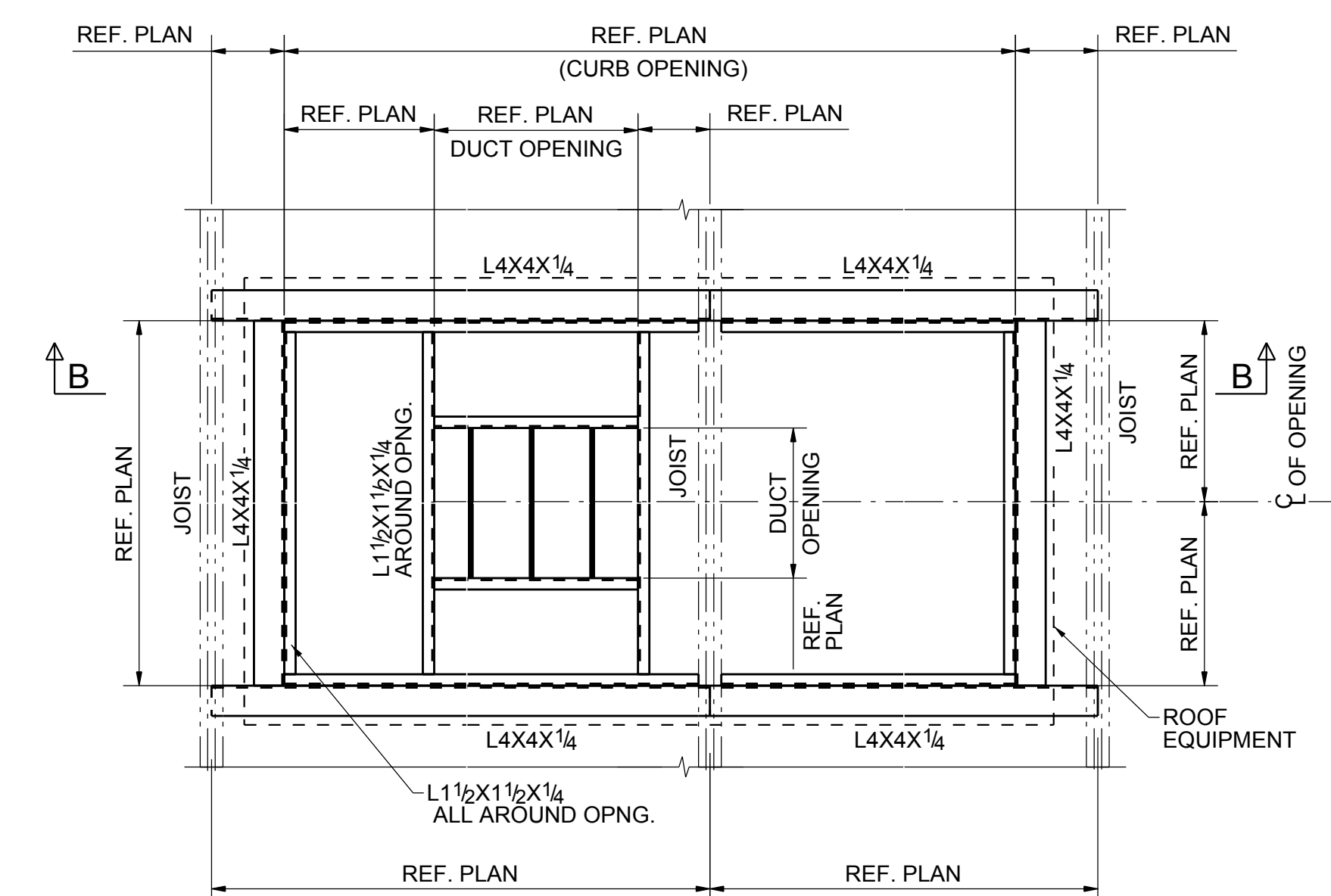
TYPICAL ROOF EQUIPMENT SUPPORT FRAME DETAIL
