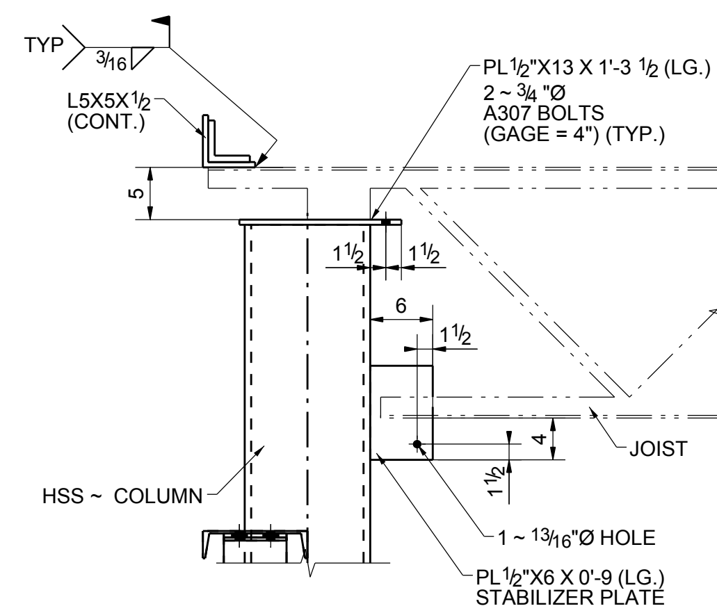
TYPICAL JOIST TO HSS ~ COLUMN TIE JOIST CONNECTION DETAIL
