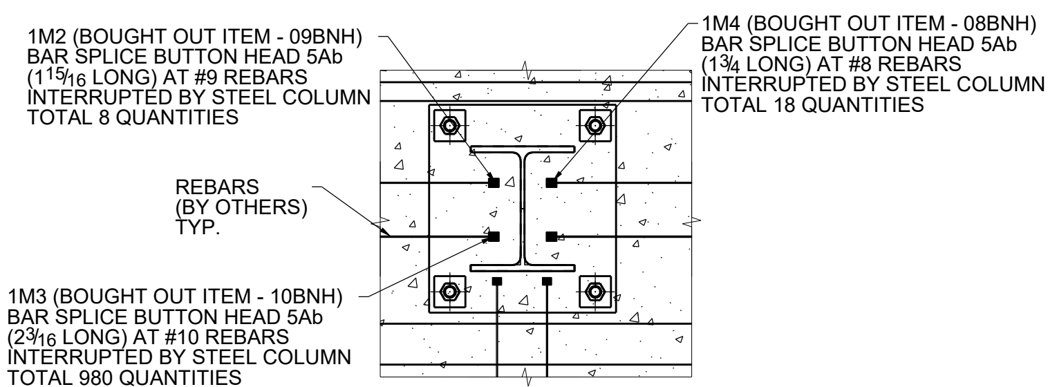
TYPICAL BAR SPLICE BUTTON HEAD 5Ab DETAIL
