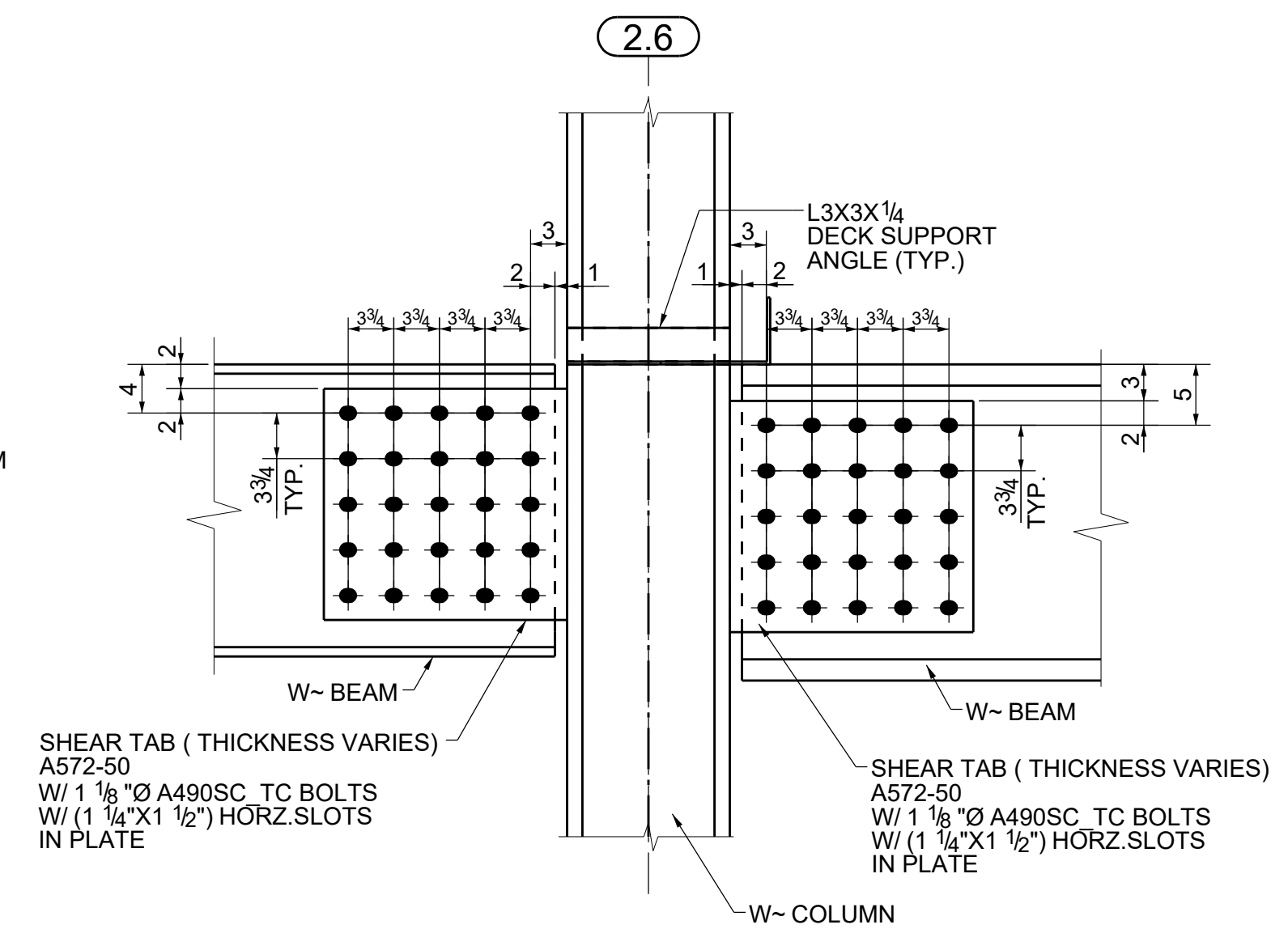
W~ BEAM TO W~COLUMN FLANGE SHEAR TAB CONNECTION
