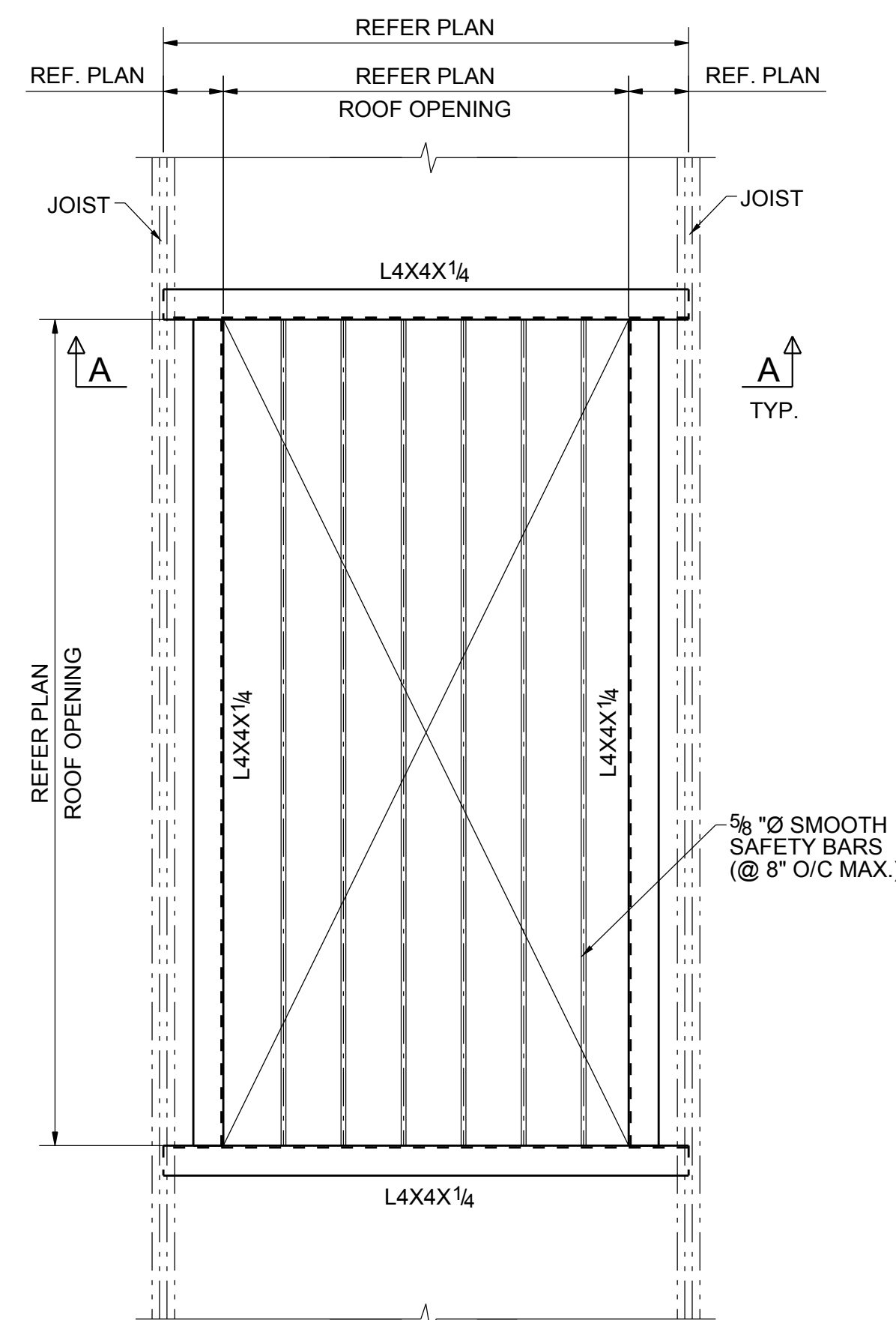
TYPICAL ROOF OPENING DECK SUPPORT DETAIL
