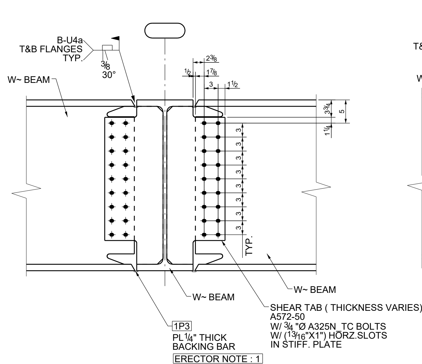
TYPICAL BEAM TO BEAM MOMENT CONNECTION DETAIL
