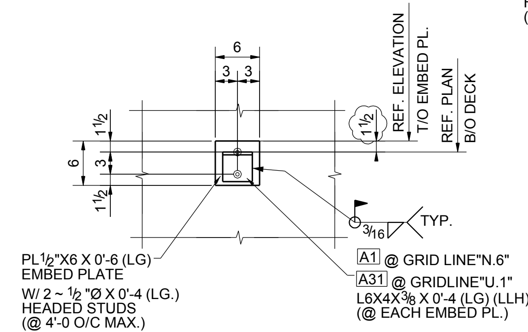
SECTION 11A - 11A
