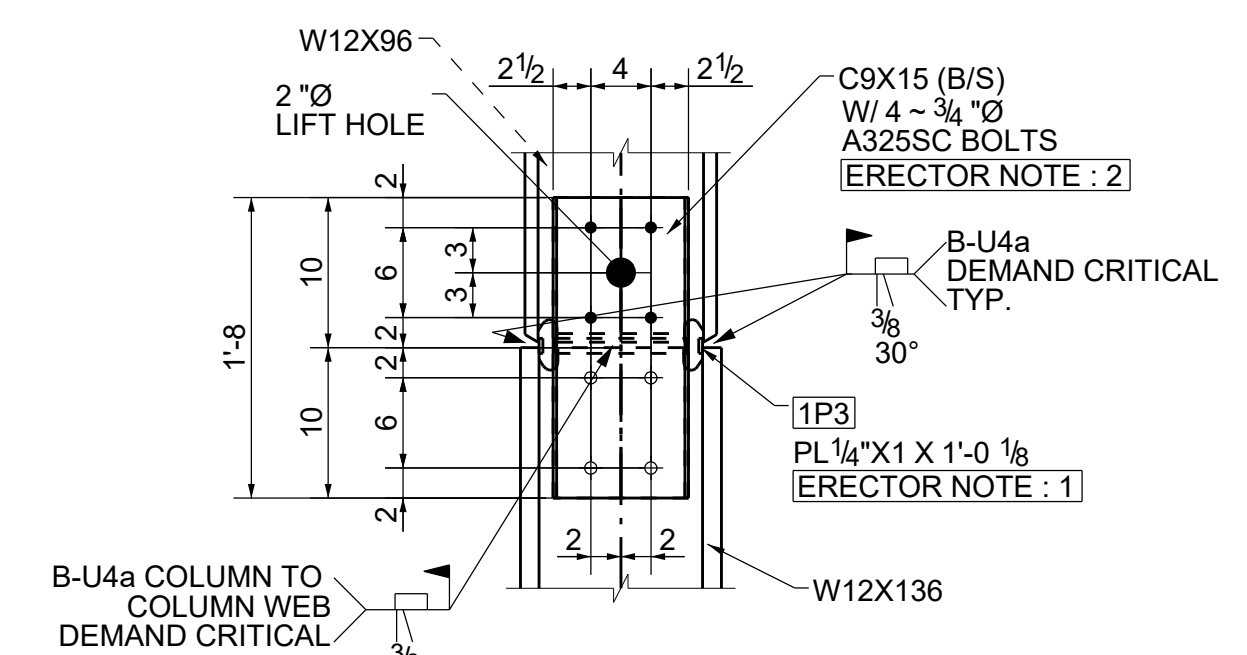
TYPICAL W12X136 COLUMN TO W12X96 COLUMN SPLICE CONNECTION DETAILS @ BRACE LOCATION
