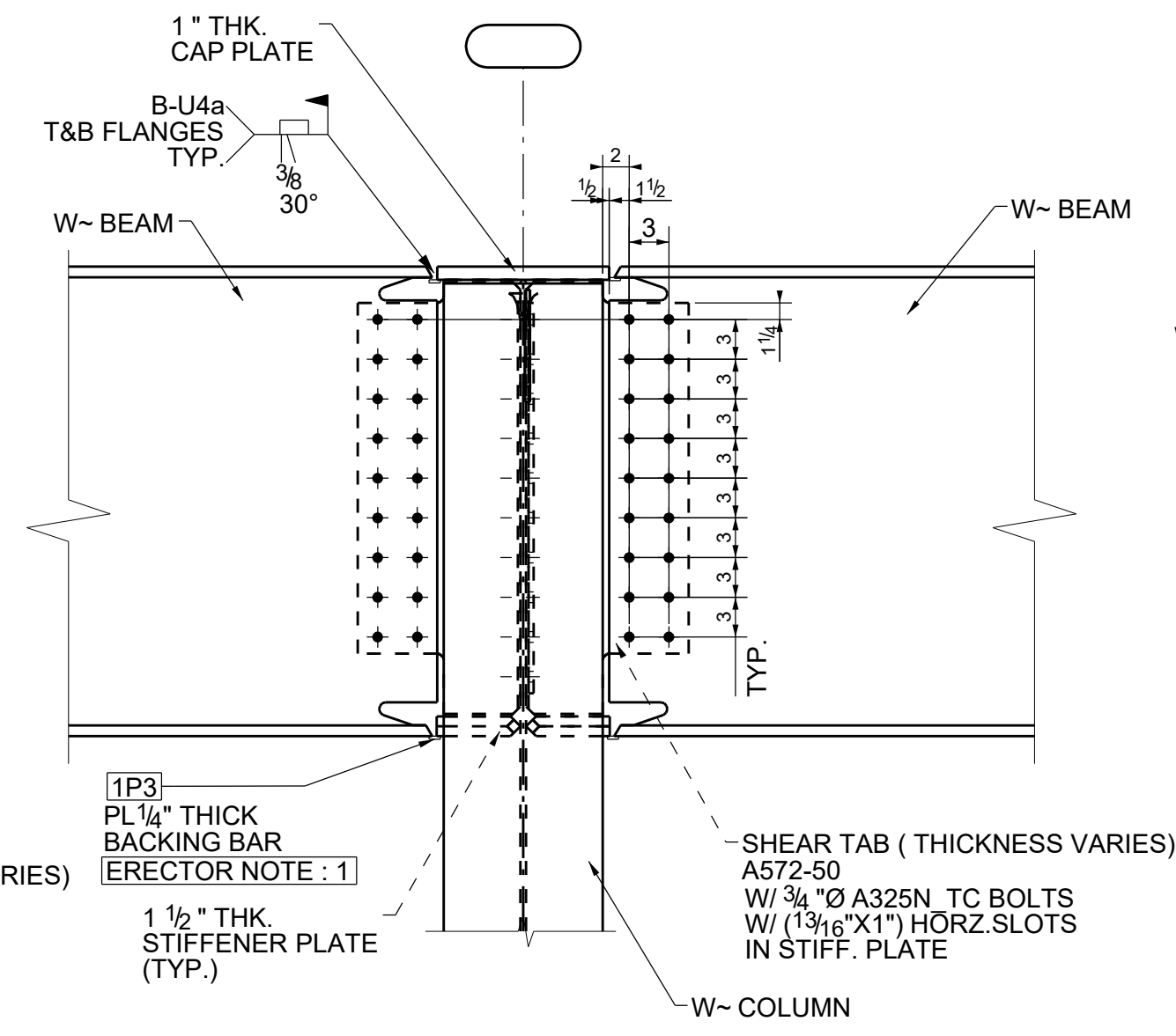
W~ BEAM TO W~COLUMN WEB MOMENT CONNECTION
