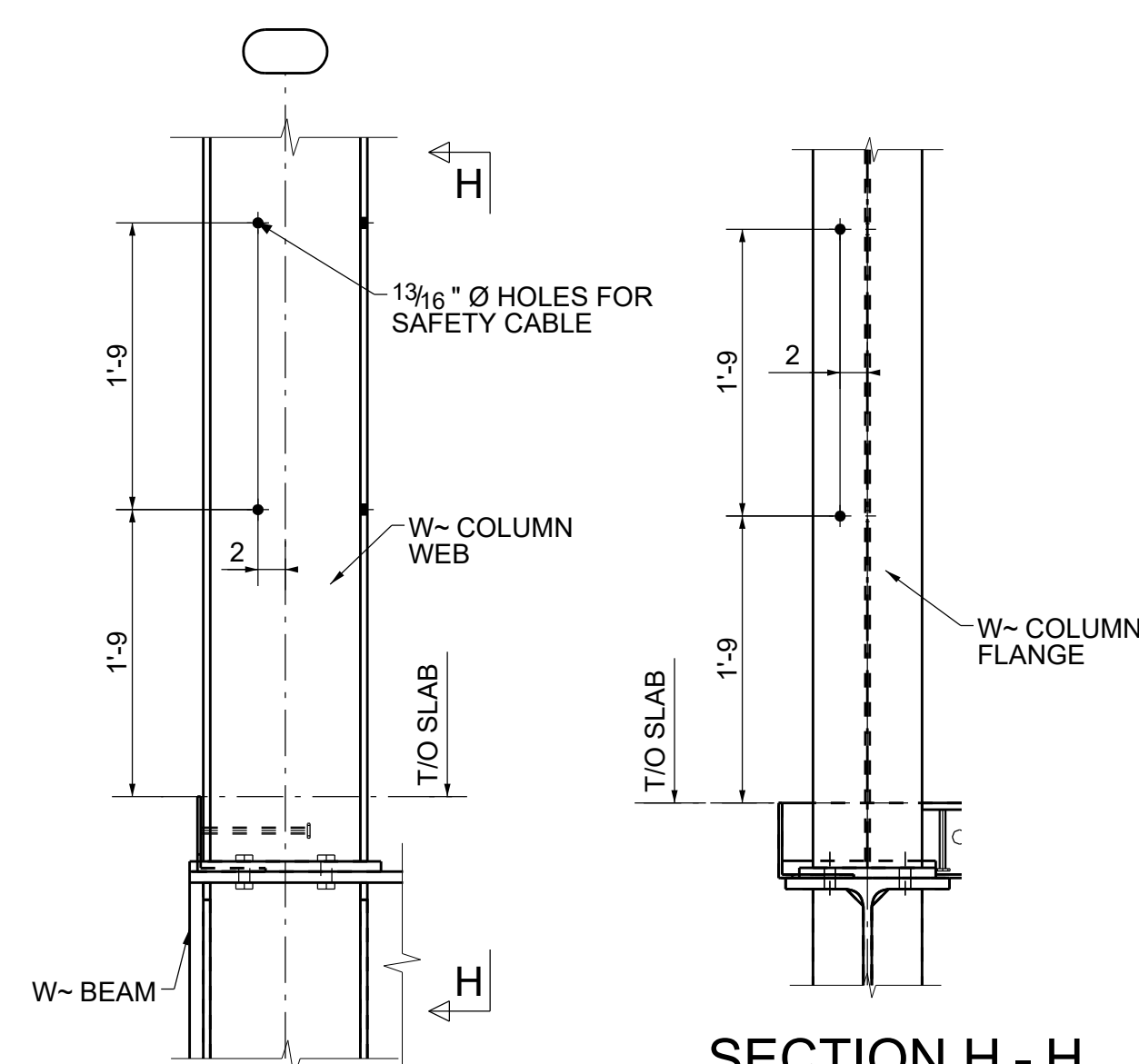
TYPICAL SAFETY CABLE HOLE DETAIL
