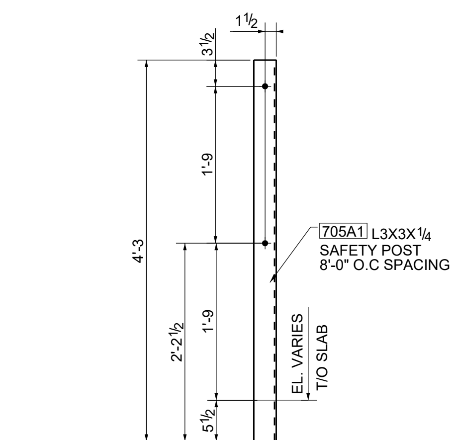
TYPICAL TEMPORARY ANGLE SAFETY CABLE POST DETAIL
