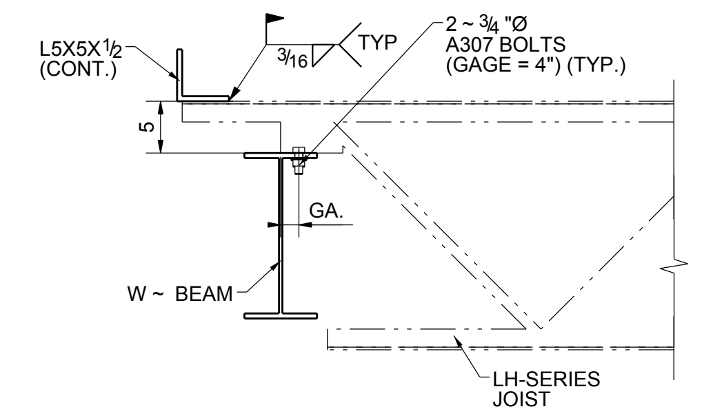
TYPICAL JOIST TO W ~ BEAM CONNECTION DETAIL
