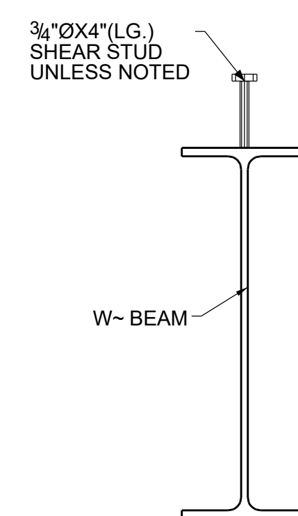
TYPICAL SHEAR STUD DETAIL
