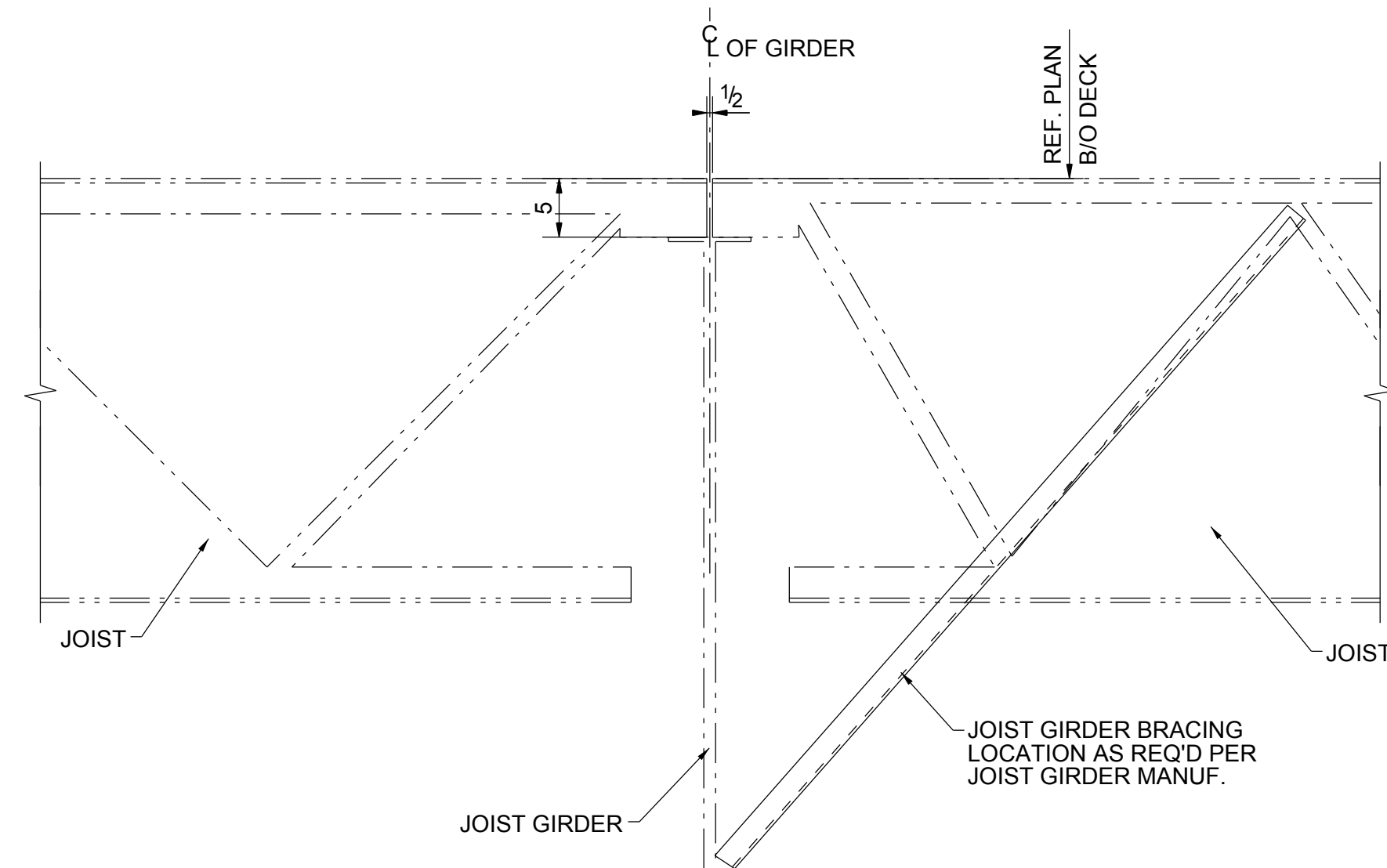
TYPICAL JOIST TO GIRDER CONNECTION DETAIL
