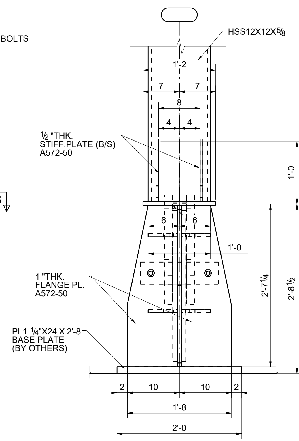
SECTION 57A - 57A
