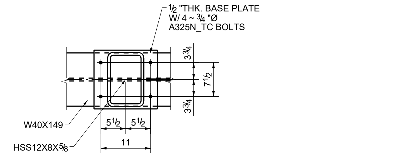
SECTION 87A - 87A
