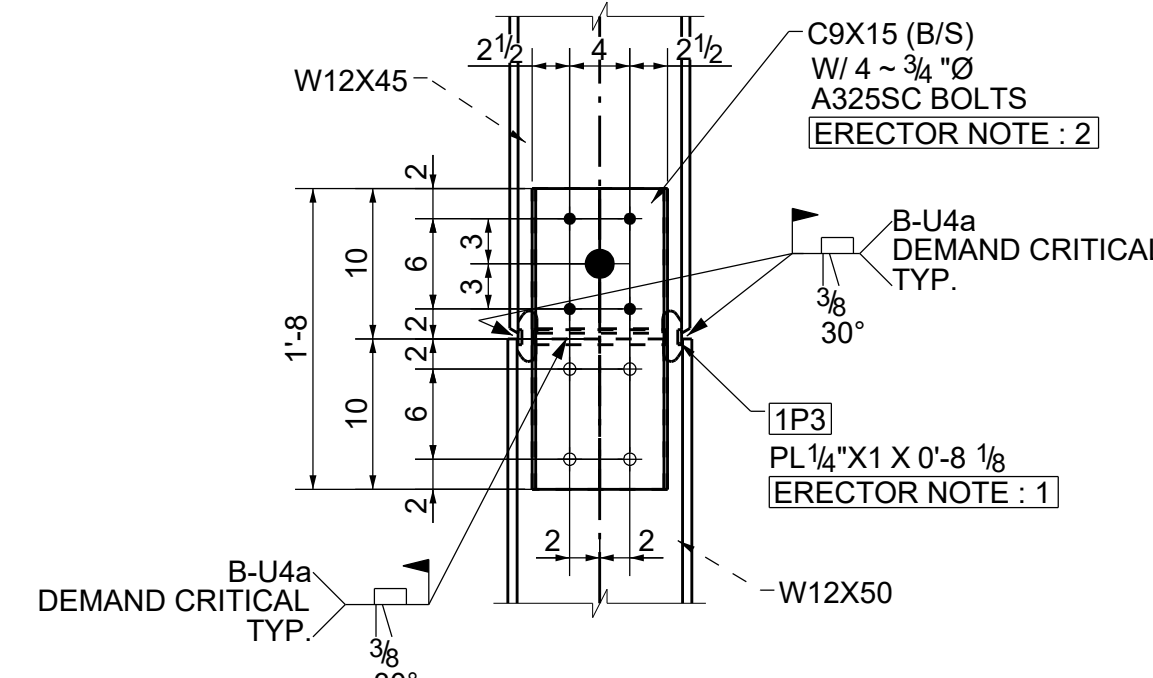
TYPICAL W12X50 COLUMN TO W12X45 COLUMN SPLICE CONNECTION DETAILS @ BRACE LOCATION
