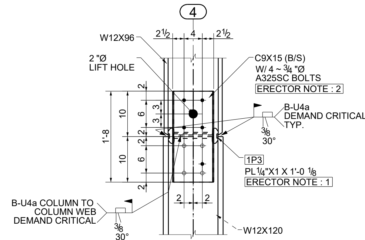
TYPICAL W12X120 COLUMN TO W12X96 COLUMN SPLICE CONNECTION DETAILS @ BRACE LOCATION
