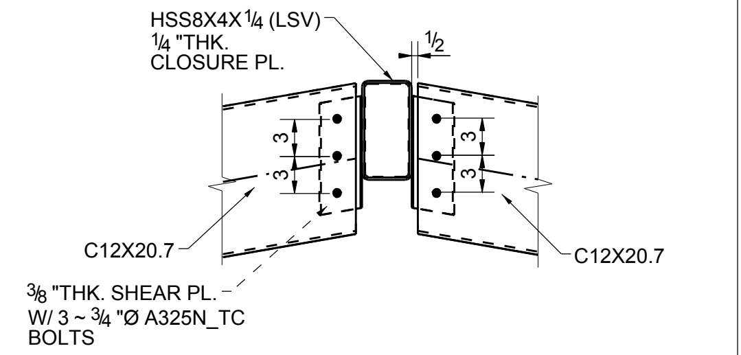
TYPICAL CHANNEL TO HSS BEAM CONNECTION DETAIL
